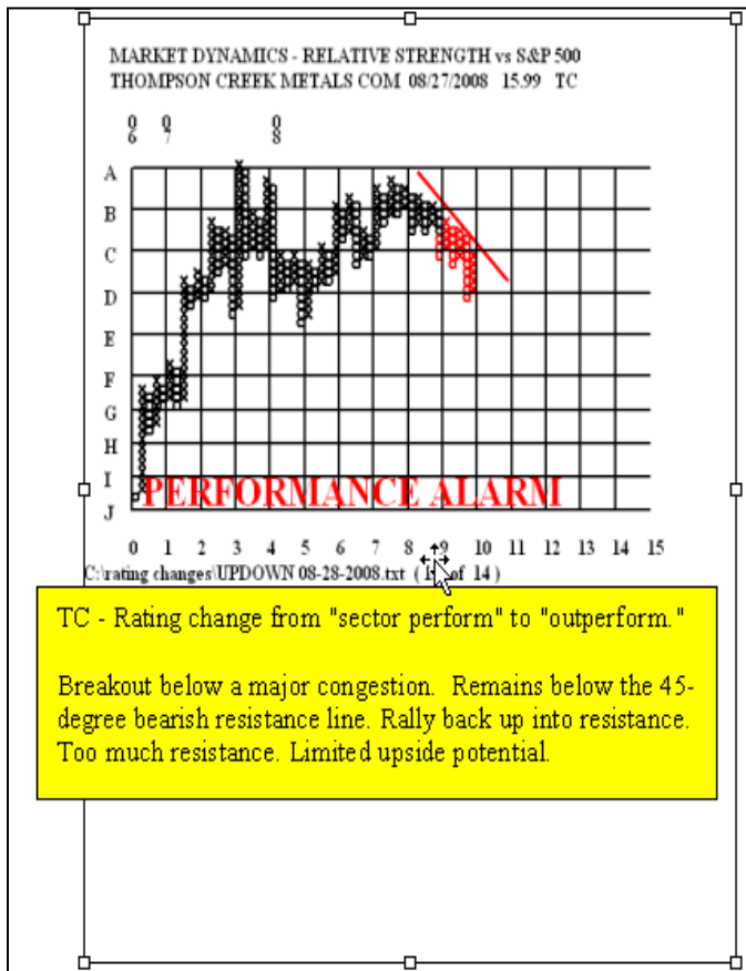
Chart from the TPARC report for 08/28/2008
